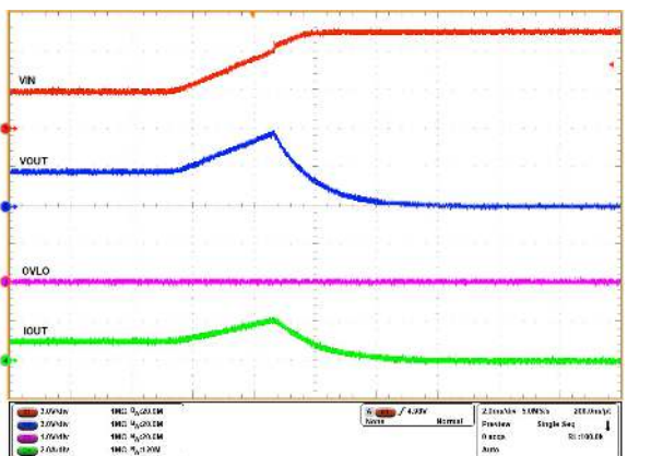
OVLO pin shorted to GND, C_{OUT} = 470 \mu\text{F} , R_{OUT} = 3.3 \Omega , V_{IN} increased from 2.7 V to 7.5 V
