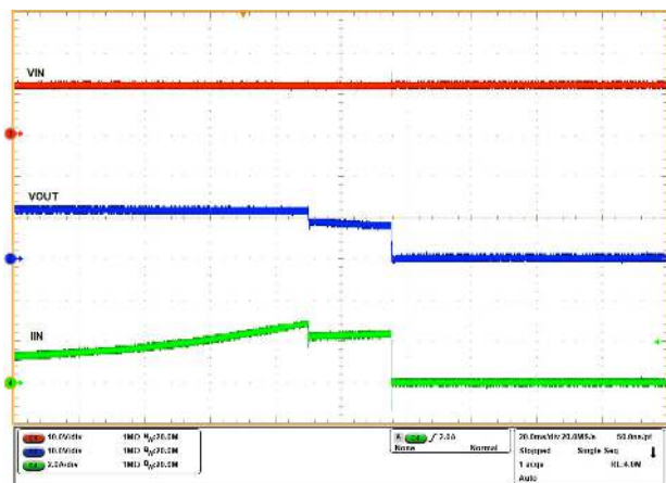
V_{IN} = 12 \text{ V} , R_{LIM} = 25 \text{ k}\Omega , load current gradually ramped up above 2.5 A
