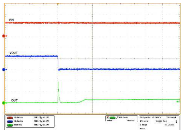
V_{IN} = 12\text{ V} , R_{ILIM} = 25\ \text{k}\Omega , OUT pin shorted to GND
