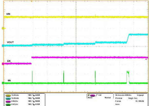
V_{IN} = 12\text{ V} , C_{OUT} = 2200\ \mu\text{F} , R_{OUT} = \text{Open} , R_{ILIM} = 25\ \text{k}\Omega , EN pin toggled from Low to High
