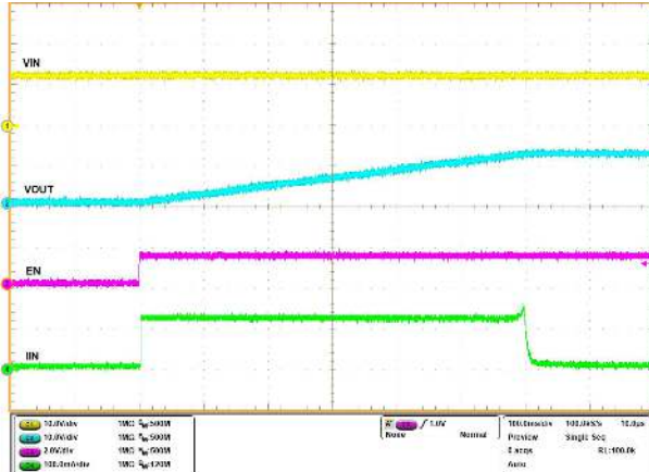
V_{IN} = 12\text{ V} , C_{OUT} = 6400\ \mu\text{F} , R_{OUT} = \text{Open} , R_{ILIM} = \text{Open} , EN pin toggled from Low to High
