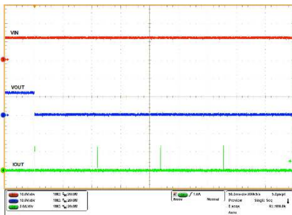
V_{IN} = 12\text{ V} , R_{ILIM} = 25\ \text{k}\Omega , OUT pin shorted to GND
