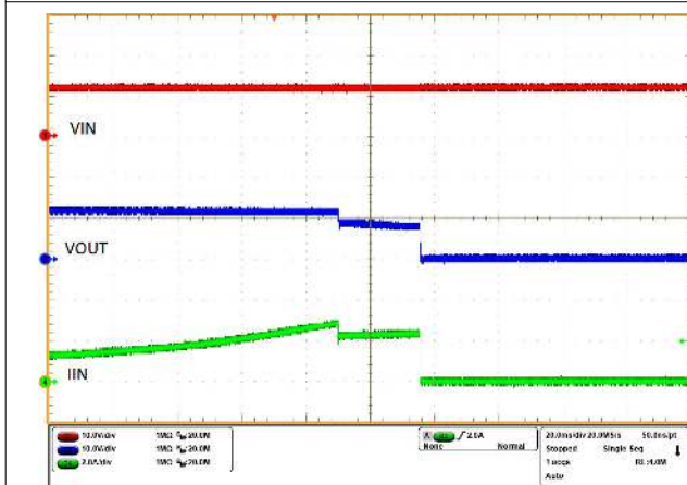
Figure 8-5. Overcurrent Protection
