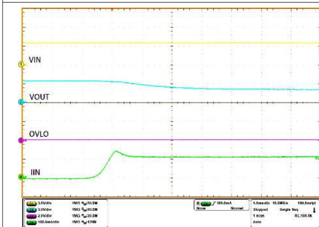
Figure 8-12. Overcurrent Protection
