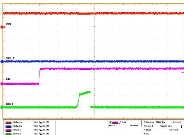
V_{IN} = 12\text{ V} , R_{ILIM} = 25\ \text{k}\Omega , EN pin toggled from Low to High with OUT pin shorted to GND
