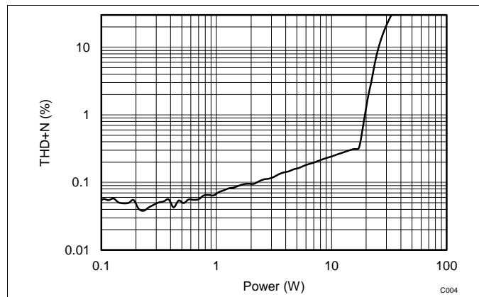
Figure 3. THD+N vs BTL Output Power at 1 kHz into 4 Ω
