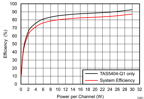
Efficiency Four Channels at 4 Ω Each
