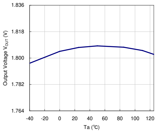
VR=1.8V
