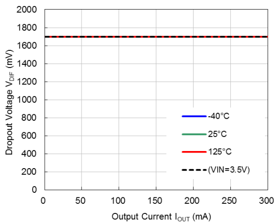
VR=1.8V
