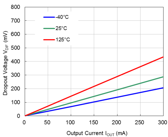
VR=5.0V
