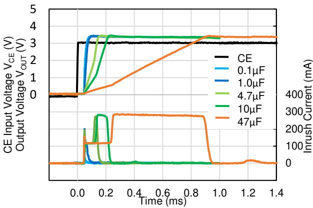
VR=5.0V, CE at rising
