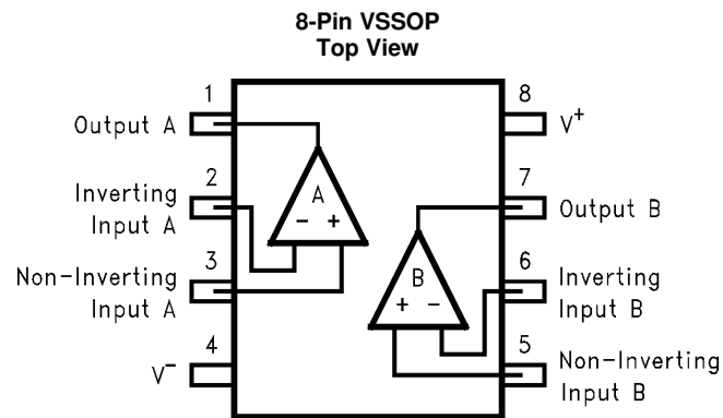
Pin Functions
