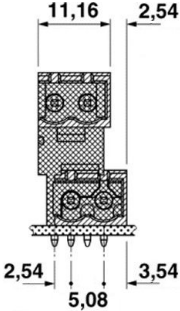
Dimensioned drawing
