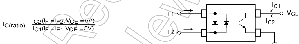
Fig.1: Collector current ratio test circuit
