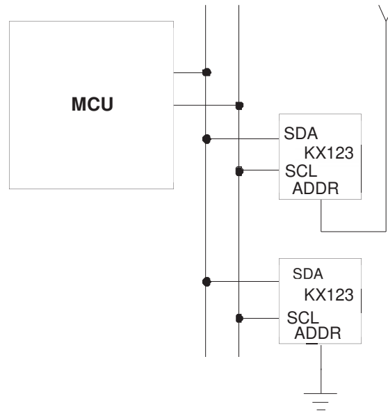
Figure 1. Multiple KX123 I 2 C Connection
