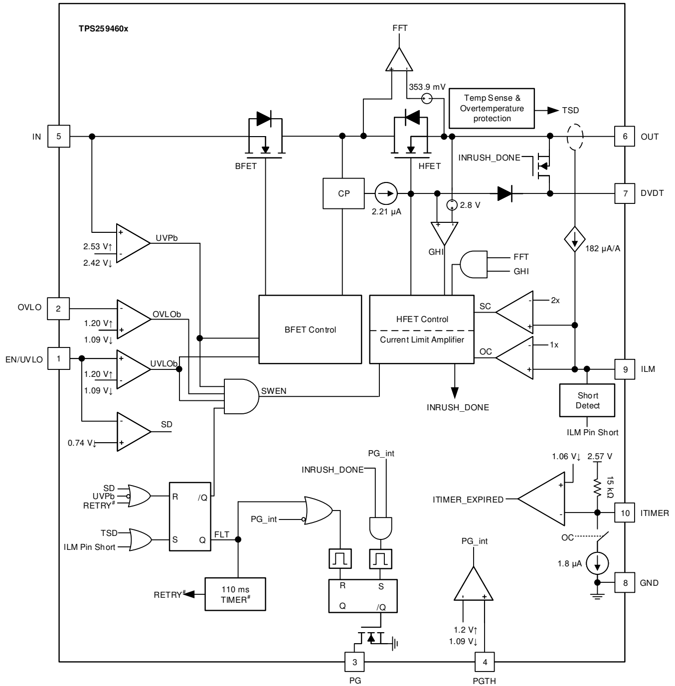
Figure 8-1. TPS259460x Block Diagram
