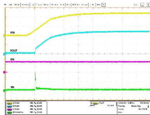
V_{EN/UVLO} = 3.3\text{ V} , C_{OUT} = 30\ \mu\text{F} , C_{dVdt} = \text{Open} , V_{IN} ramped up to 12 V
