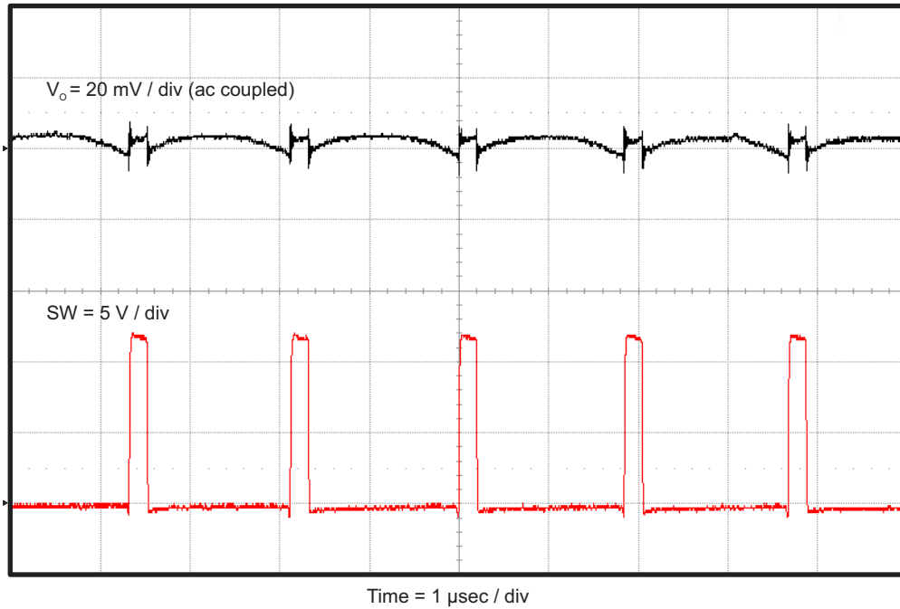
Figure 4-7. TPS563219AEM-663 Output Voltage Ripple, I_{OUT} = 3 \text{ A}
