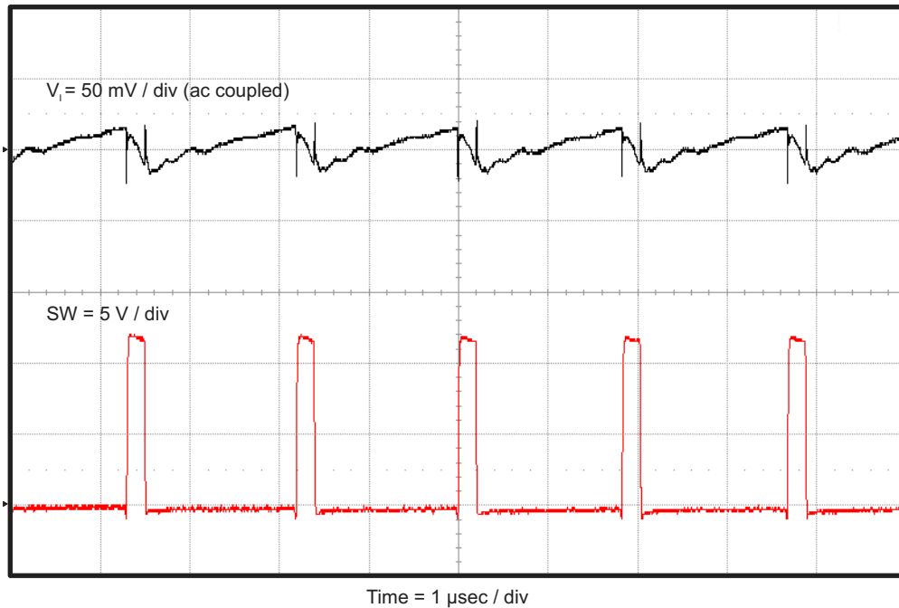
Figure 4-8. TPS563219AEM-663 Input Voltage Ripple, I_{OUT} = 3 \text{ A}
