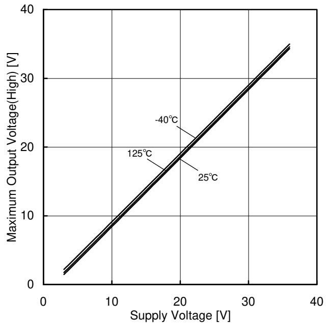
Figure 5. Maximum Output Voltage(High) vs Supply Voltage ( R_L=10k\Omega )
