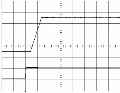
Start-up enabled by connecting V_i at: T_{ref} = +25^{\circ}\text{C} , I_O = 22\text{ A} resistive load, V_i = 5.0\text{ V} . Top trace: output voltage (0.5 V/div.). Bottom trace: input voltage (5 V/div.). Time scale: 5 ms/div..
