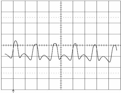
Output voltage ripple (20mV/div.) at: T_{ref} = +25^\circ\text{C} , I_O = 22\text{ A} resistive load, V_i = 5.0\text{ V} . Time scale: 2 \mu\text{s}/\text{div} . See the filter in the Output ripple and noise section (EMC Specification).
