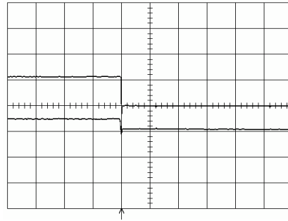
Shut-down enabled by disconnecting V_i at: T_{ref} = +25^\circ\text{C} , I_O = 22\text{ A} resistive load, V_i = 5.0\text{ V} . Top trace: output voltage (1.0 V/div.). Bottom trace: input voltage (2 V/div.). Time scale: 5.0 ms/div..
