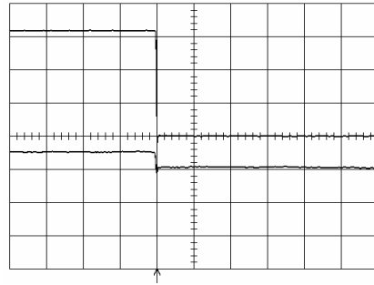
Shut-down enabled by disconnecting V_i at: T_{ref} = +25^{\circ}\text{C} , I_O = 22\text{ A} resistive load, V_i = 5.0\text{ V} .. Top trace: output voltage (1.0 V/div.). Bottom trace: input voltage (2 V/div.). Time scale: 5.0 ms/div..
