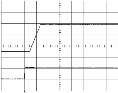
Start-up enabled by connecting V_i at: T_{ref} = +25^\circ\text{C} , I_O = 22\text{ A} resistive load, V_i = 5.0\text{ V} . Top trace: output voltage (0.5 V/div.). Bottom trace: input voltage (5 V/div.). Time scale: 5 ms/div..
