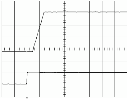
S Start-up enabled by connecting V_i at: T_{ref} = +25^{\circ}\text{C} , I_O = 22\text{ A} resistive load, V_i = 5.0\text{ V} .. Top trace: output voltage (1.0 V/div.). Bottom trace: input voltage (5 V/div.). Time scale: 5 ms/div..
