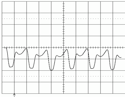
Output voltage ripple (20mV/div.) at: T_{ref} = +25^{\circ}\text{C} , I_O = 22\text{ A} resistive load, V_i = 5.0\text{ V} . Time scale: 2 \mu\text{s} /div. See the filter in the Output ripple and noise section (EMC Specification).
