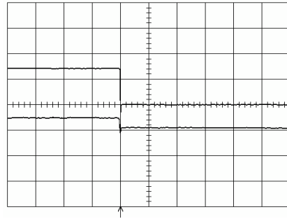
Shut-down enabled by disconnecting V_i at: T_{ref} = +25^{\circ}\text{C} , I_O = 22\text{ A} resistive load, V_i = 5.0\text{ V} . Top trace: output voltage (1.0 V/div.). Bottom trace: input voltage (2 V/div.). Time scale: 5.0 ms/div..
