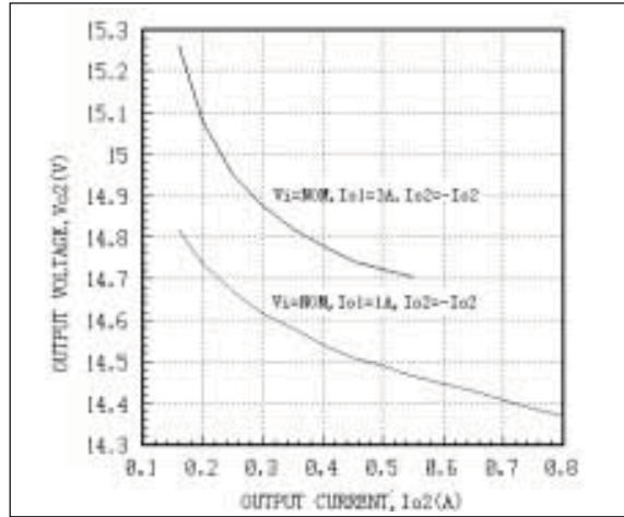
Fig. 26 AEW05ACC48 Load Regulation Curves Tc=25°C
