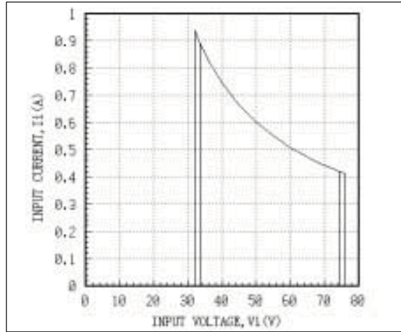
Fig. 14 AEW05ACC48 Input Characteristic Curves
