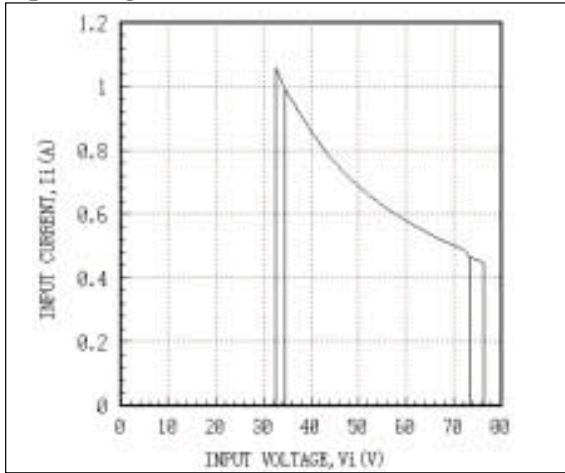
Fig. 13 AEW05ABB48 Input Characteristic Curves
