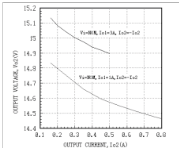
Fig. 24 AEW05ACC24 Load Regulation Curves Tc=25°C
