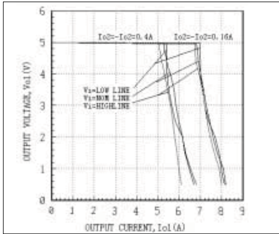
Fig. 21 AEW05ABB48 Main Output Character Curves Tc=25°C
