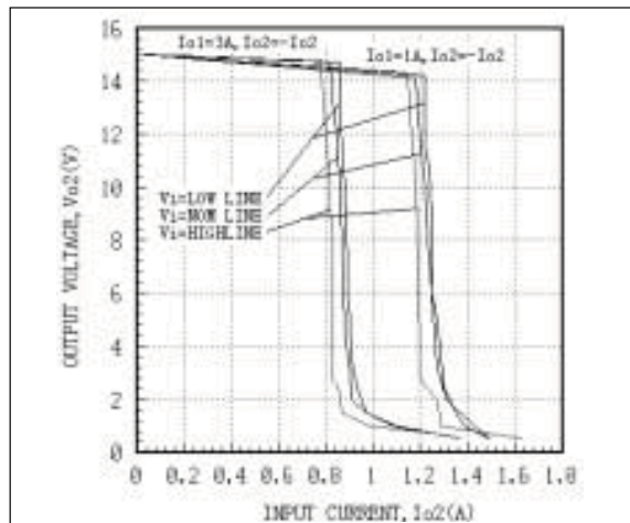
Fig. 18 AEW05ACC48 Auxiliary output Character Curves
