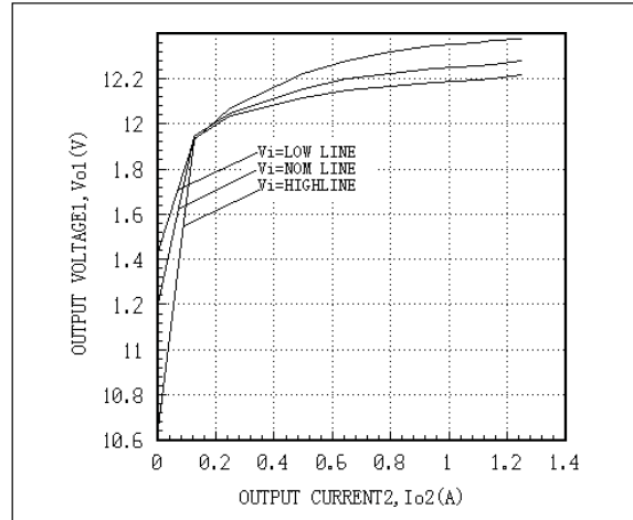
Fig. 32 AEW01BB24 Cross Regulation Io2=10%Io constant, Io1 variable, Tc=25°C
