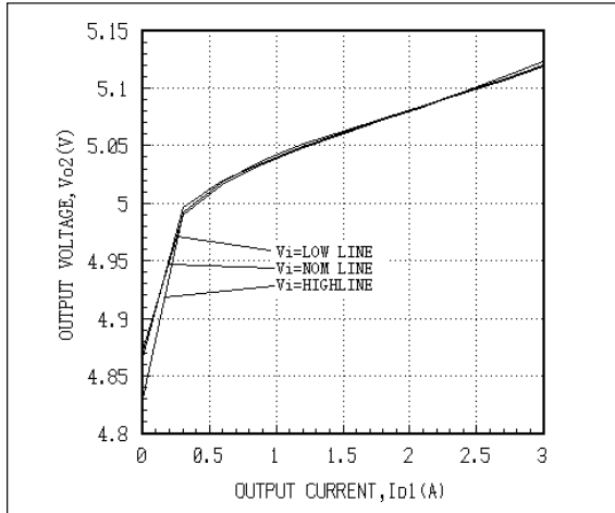
Fig. 31 AEW03AA24 Cross Regulation Io2=10%Io constant, Io1 variable, Tc=25°C
