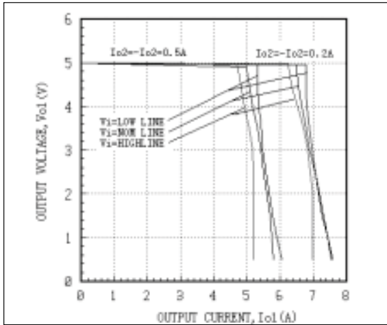
Fig. 15 AEW05ABB24 Main Output Character Curves
