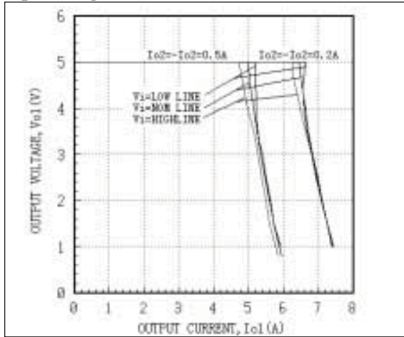
Fig. 19 AEW05ABB24 Main Output Character Curves Tc=25°C
