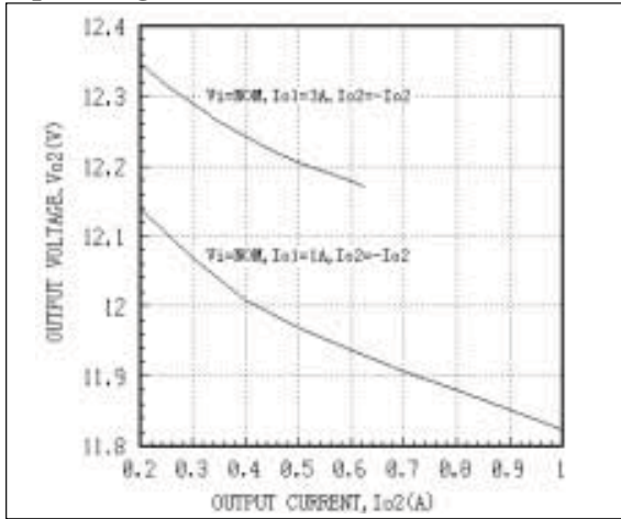
Fig. 25 AEW05ABB48 Load Regulation Curves Tc=25°C
