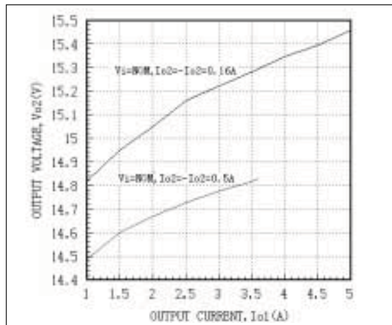
Fig. 30 AEW05ACC48 Cross Regulation Curves Tc=25°C
