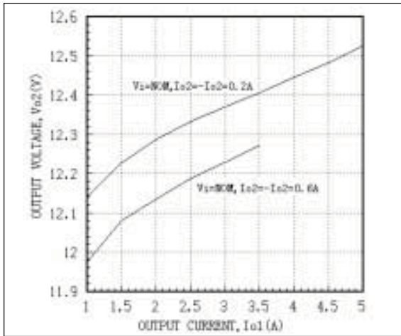
Fig. 29 AEW05ABB48 Cross Regulation Curves Tc=25°C
