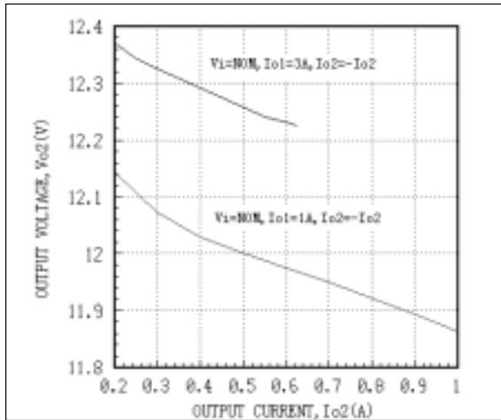
Fig. 23 AEW05ABB24 Load Regulation Curves Tc=25°C
