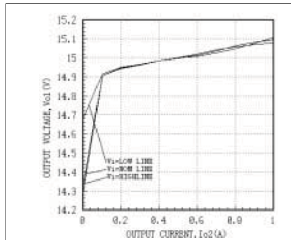
Fig. 36 AEW01CC48 Cross Regulation Io2=10%Io constant, Io1 variable, Tc=25°C
