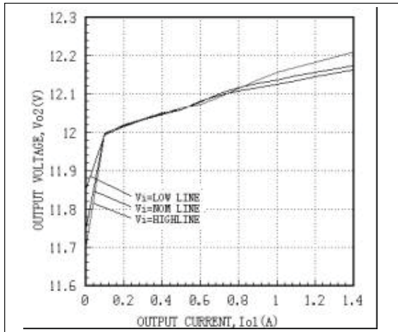
Fig. 35 AEW01BB48 Cross Regulation Io2=10%Io constant, Io1 variable, Tc=25°C
