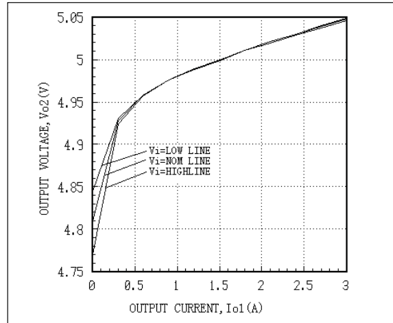
Fig. 34 AEW03AA48 Cross Regulation Io2=10%Io constant, Io1 variable, Tc=25°C
