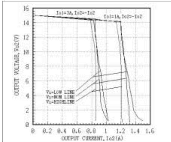
Fig. 22 AEW05ACC48 Auxiliary output Character Curves Tc=25°C
