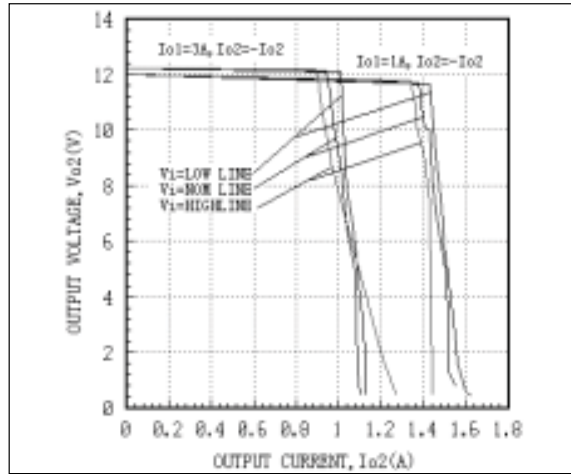
Fig. 16 AEW05ACC24 Auxiliary output Character Curves
