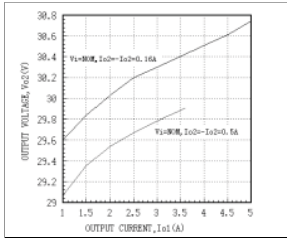
Fig. 28 AEW05ACC24 Cross Regulation Curves Tc=25°C
