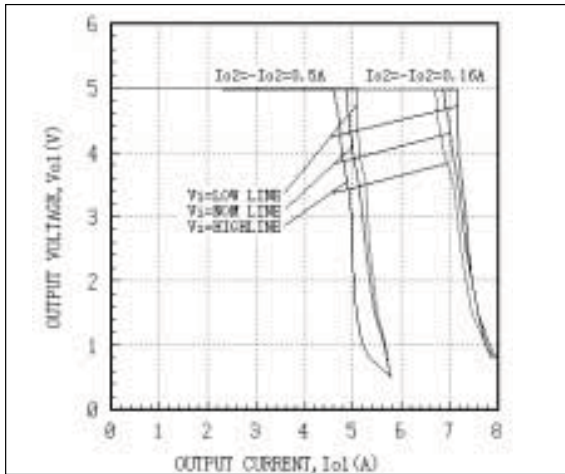
Fig. 17 AEW05ABB48 Main Output Character Curves
