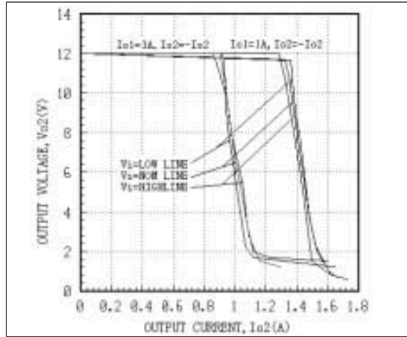
Fig. 20 AEW05ACC24 Auxiliary output Character Curves Tc=25°C
