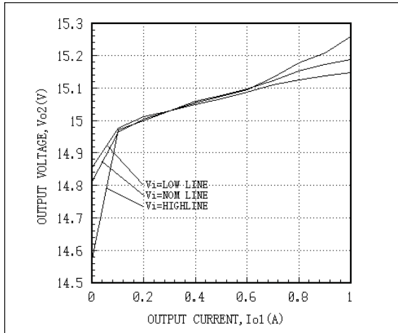
Fig. 33 AEW01CC24 Cross Regulation Io2=10%Io constant, Io1 variable, Tc=25°C
