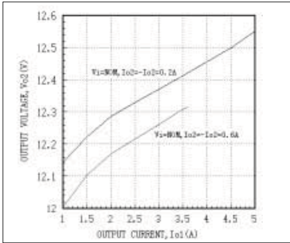
Fig. 27 AEW05ABB24 Cross Regulation Curves Tc=25°C
