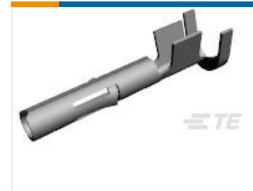
TE Part #350874-1 UMNL SOK 18-14 .0126 PTPBR
