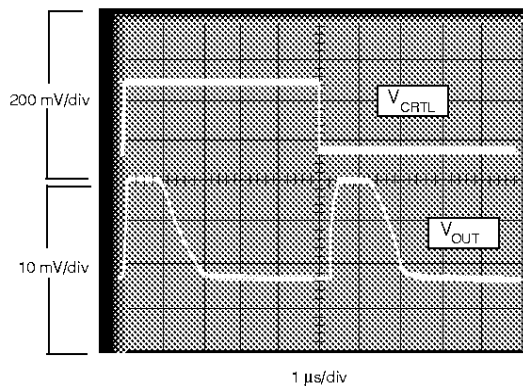
Fig. 11b Switching Transient
