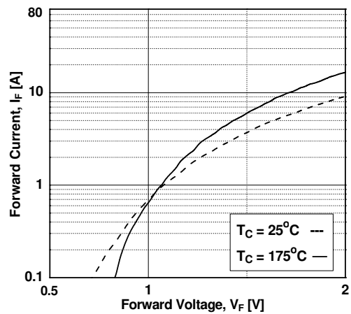
Figure 18. Forward Characteristics
