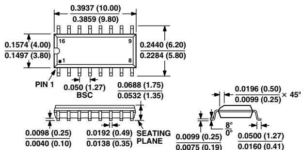
16-Lead Narrow SOIC (R-16N)
