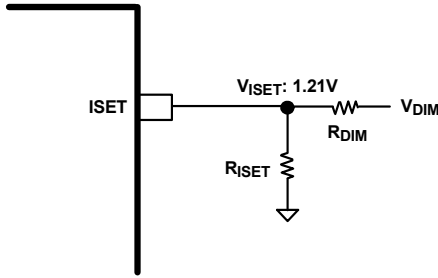
FIGURE 17. LED CURRENT CONTROL WITH V_{DIM}
