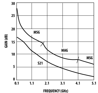
Figure 8. Gain vs. Frequency at V_{CE} = 2.7 V , I_C = 2 mA .
