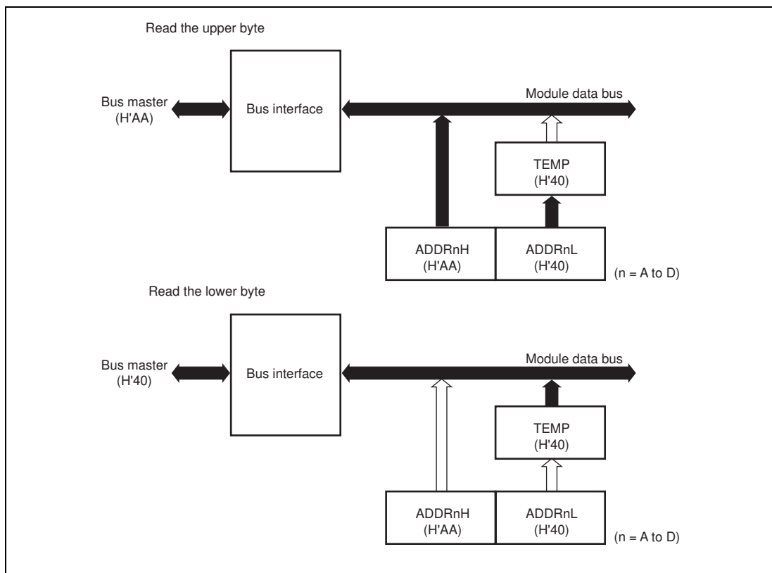
Figure 15.2 Access to ADDR (When Reading H'AA40)
