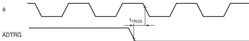
Figure 22.17 A/D Converter External Trigger Input Timing
