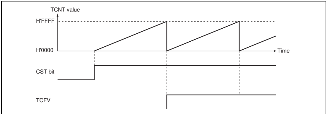
Figure 9.7 Free-Running Counter Operation
