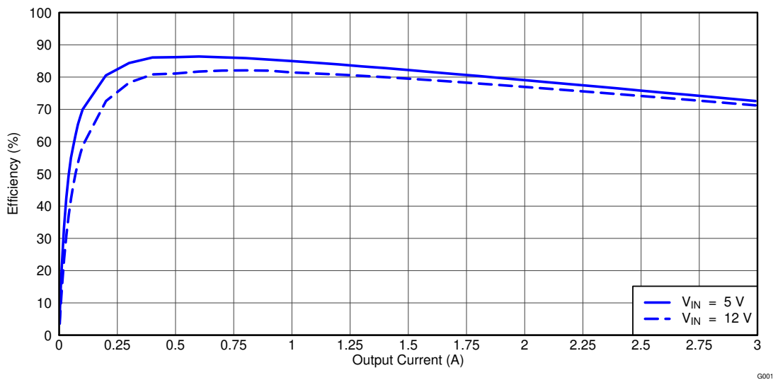
Figure 4-1. TPS54329EVM-056 Efficiency
