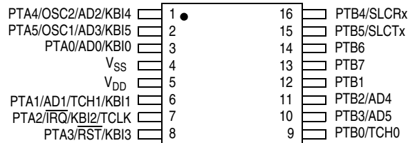
16-PIN ASSIGNMENT MC68HC908QL4 AND MC68HC908QL2 TSSOP
