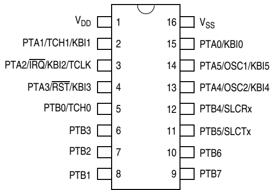
16-PIN ASSIGNMENT MC68HC908QL3 SOIC
