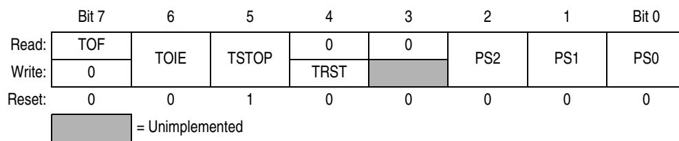
Figure 15-4. TIM Status and Control Register (TSC)
