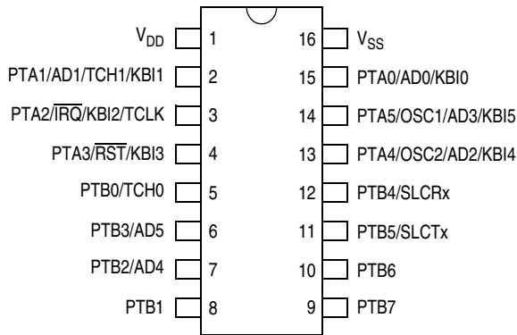
16-PIN ASSIGNMENT MC68HC908QL4 AND MC68HC908QL2 SOIC
