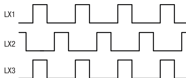
Figure 18. Out-of-Phase Operation
