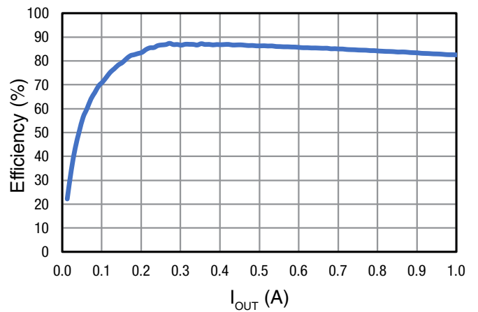
Figure 10. Efficiency Channel 2, 5V_{IN} 1.5V_{OUT}
