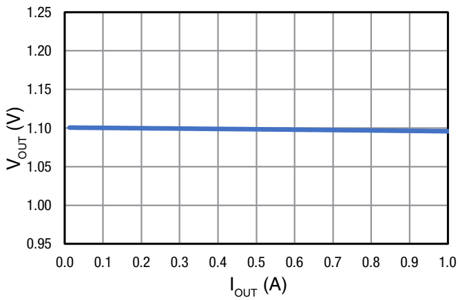
Figure 3. Load Regulation Channel 1, 5V_{IN} , 1.1V_{OUT}
