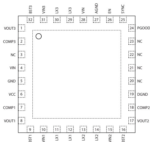
Figure 2. XR77103-G1R2 Pinout
