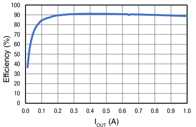
Figure 12. Efficiency Channel 3, 5V_{IN} 3.3V_{OUT}
