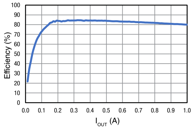
Figure 8. Efficiency Channel 1, 5V_{IN} 1.1V_{OUT}
