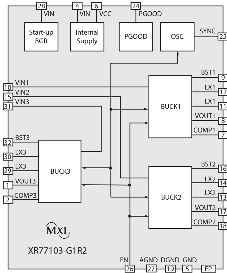
Figure 17. Functional Block Diagram
