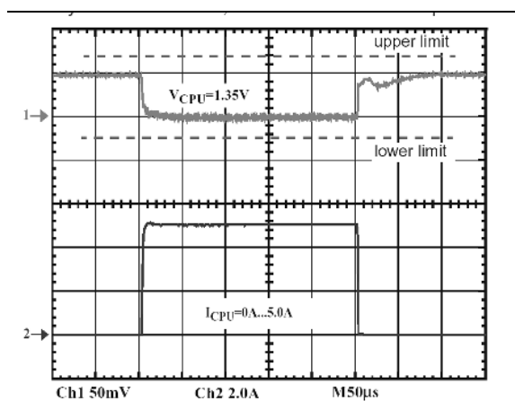
Figure 8. Converter Response to 5A Load Step
