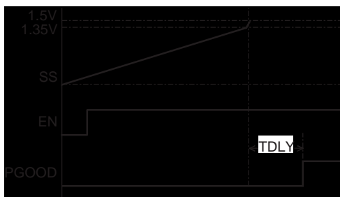
Figure 3. Soft-Start function
