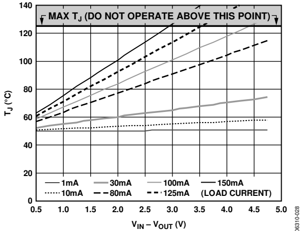
Figure 28. 0 mm 2 of PCB Copper, T A = 50°C
