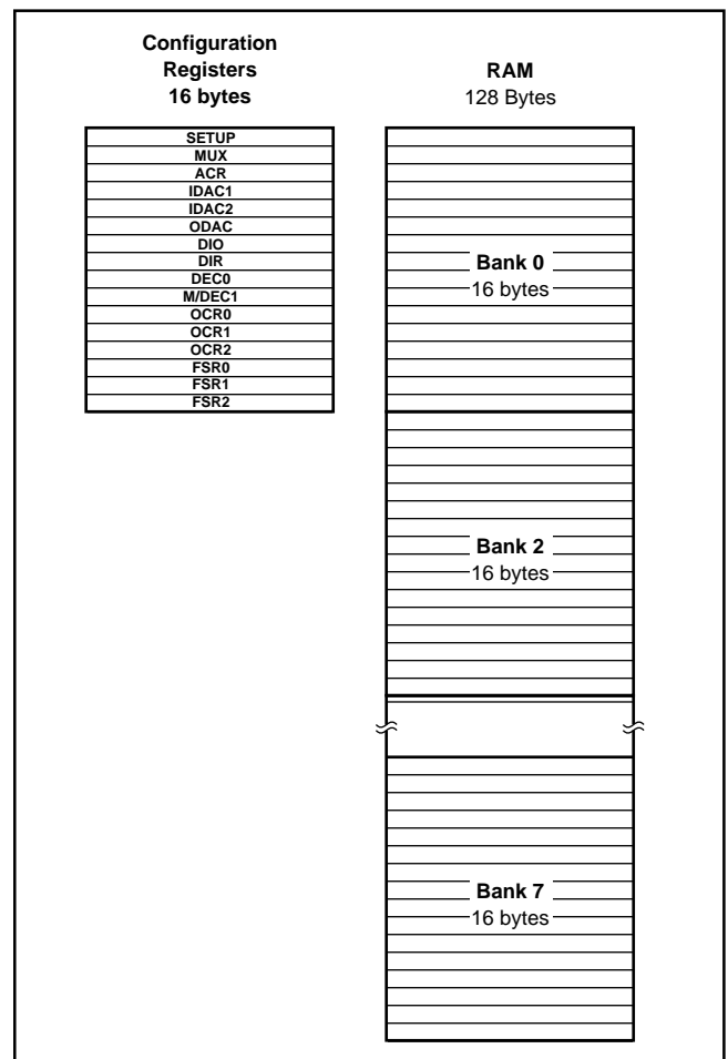
FIGURE 5. Memory Organization.
