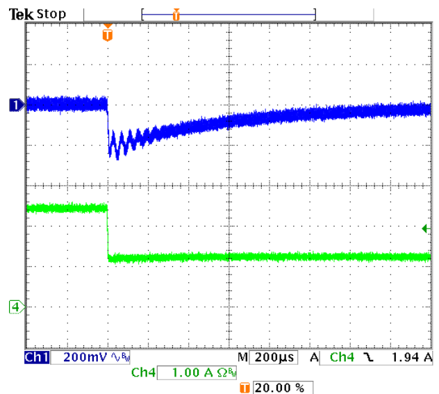
Fig. 7: Output voltage response for V_{out} = -7.5V to negative load current step change from 2.5A to 1.25A with slew rate of -5A/us at V_{in} = 24V . C_{in} = 20\mu F , C_o = 22\mu F ceramic.
