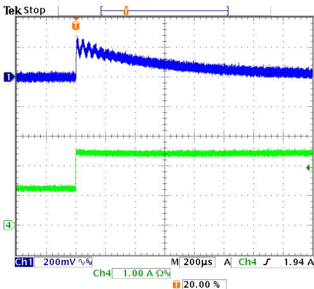
Fig. 6: Output voltage response for V_{out} = -7.5V to positive load current step change from 1.25A to 2.5A with slew rate of 5A/us at V_{in} = 24V . C_{in} = 20\mu F , C_o = 22\mu F ceramic.
