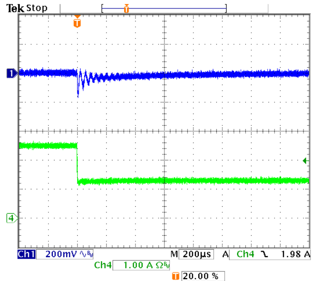
Fig. 11: Output voltage response for V_{out} = -2.5V to negative load current step change from 2.5A to 1.25A with slew rate of -5A/us at V_{in}=24V . C_{in}=40\mu F , C_o=22\mu F ceramic. Top trace: V_{out} (200mV/div.) Bottom trace: load current (1A/div.) Time scale: 200us/div.
