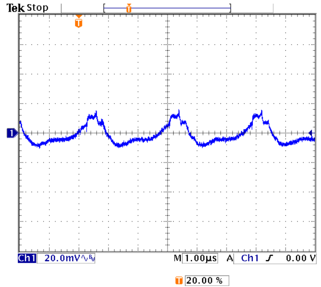
Fig. 9: Output voltage ripple (20mV/div.) for V_{out} = -2.5V at full rated load current into a resistive load. C_{in}=40\mu F , C_o=22\mu F ceramic at V_{in}=24V . Blue trace: V_{out} (20mV/div.) Time scale: 1 us/div.
