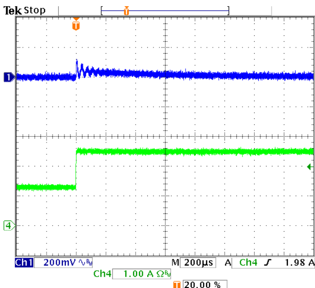
Fig. 10: Output voltage response for V_{out} = -2.5V to positive load current step change from 1.25A to 2.5A with slew rate of 5A/us at V_{in}=24V . C_{in}=40\mu F , C_o=22\mu F ceramic. Top trace: V_{out} (200mV/div.) Bottom trace: load current (1A/div.) Time scale: 200us/div.
