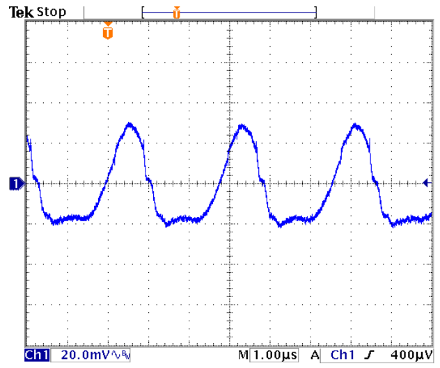
Fig. 5: Output voltage ripple (20mV/div.) for V_{out} = -7.5V at full rated load current into a resistive load. C_{in} = 20\mu F , C_o = 22\mu F ceramic at V_{in} = 24V .
