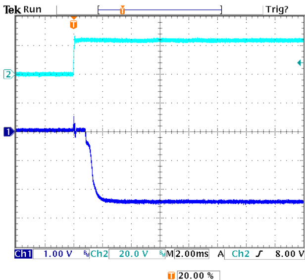
Fig. 8: Turn-on transient for V_{out} = -2.5V with application of V_{in} at full rated load current into a resistive load. C_{in}=20\mu F , C_o=22\mu F ceramic at V_{in}=24V . Top trace: V_{in} (20V/div.) Bottom trace: V_{out} (1V/div.) Time scale: 2 ms/div.
