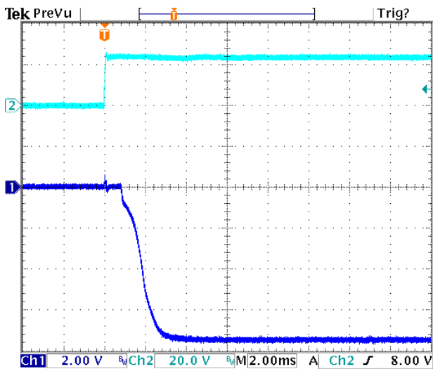
Fig. 4: Turn-on transient for V_{out} = -7.5V with application of V_{in} at full rated load current into resistive load. C_{in} = 20\mu F , C_o = 22\mu F ceramic at V_{in} = 24V .
