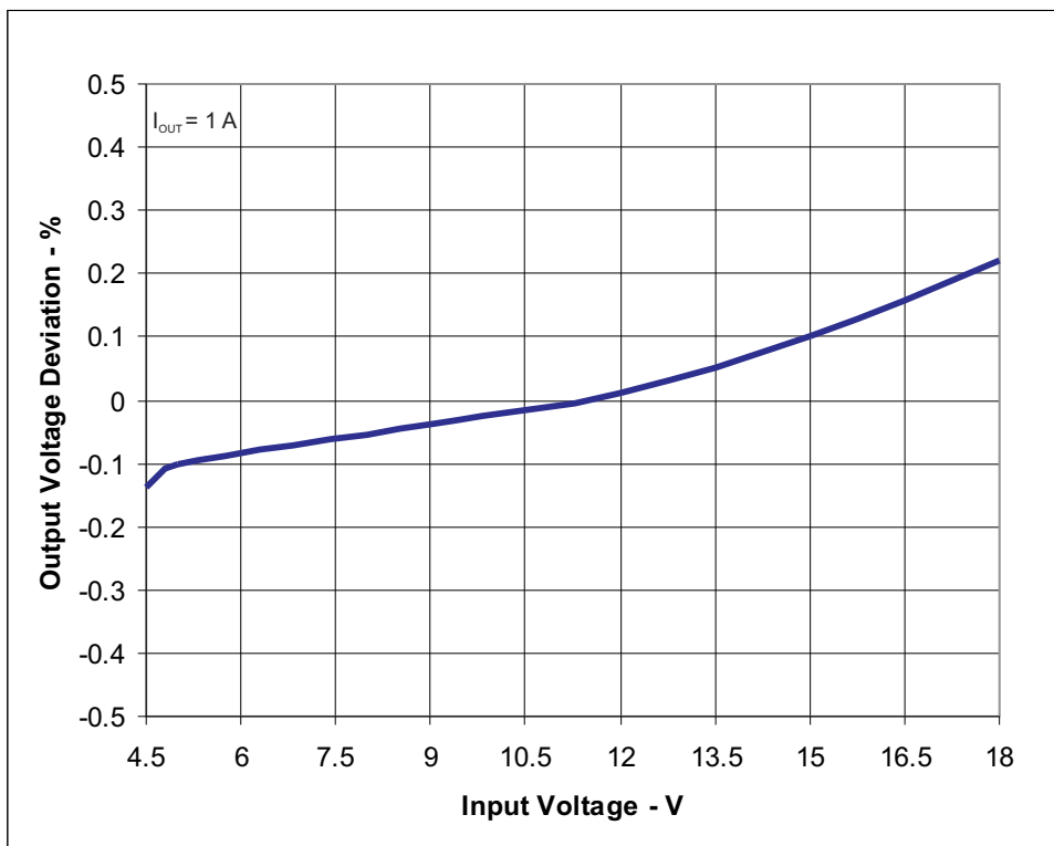
Figure 4-5. TPS54227EVM-686 Line Regulation
