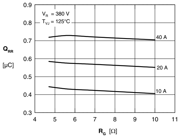
Fig. 15 Reverse recovery charge Q_{RR} I_{RM} of the boost diode versus R_G
