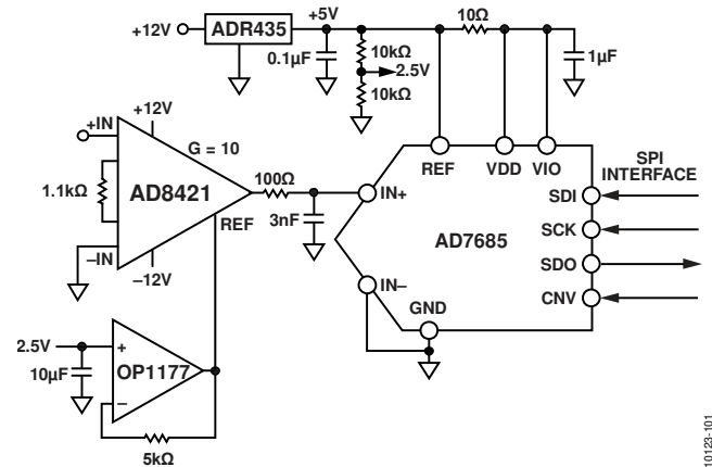
Figure 1. AD8421 Driving 16-Bit AD7685
