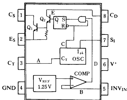
Fig. 1 Block Diagram
