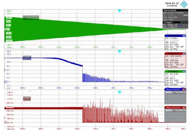
Figure 93 – Brown-out Test.
