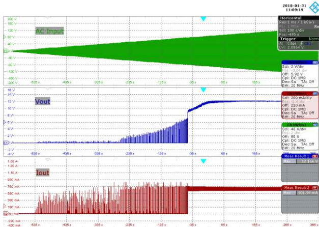
Figure 92 – Brown-in Test.
