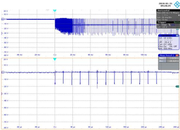
Figure 88 – 90 VAC 60 Hz, No-Load. CH1: V_{FWL\_Diode} - 10 V / div., 20 ms / div. Zoom: 40 \mu s / div. PIV_{MAX} = 36.929 V.
