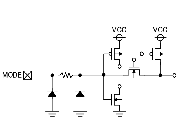
< MODE Pin >
