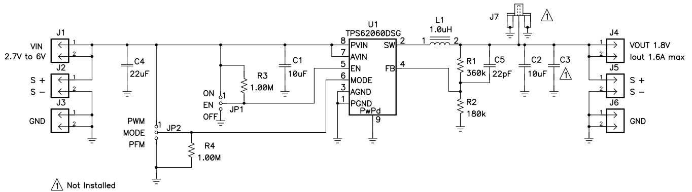
Figure 1. TPS62060EVM Schematic
