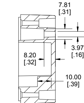
SECTION C-C MOUNTING HOLE
