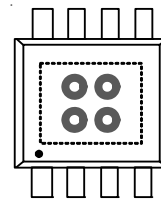
Figure 4. Standard PTH to GND Plane
