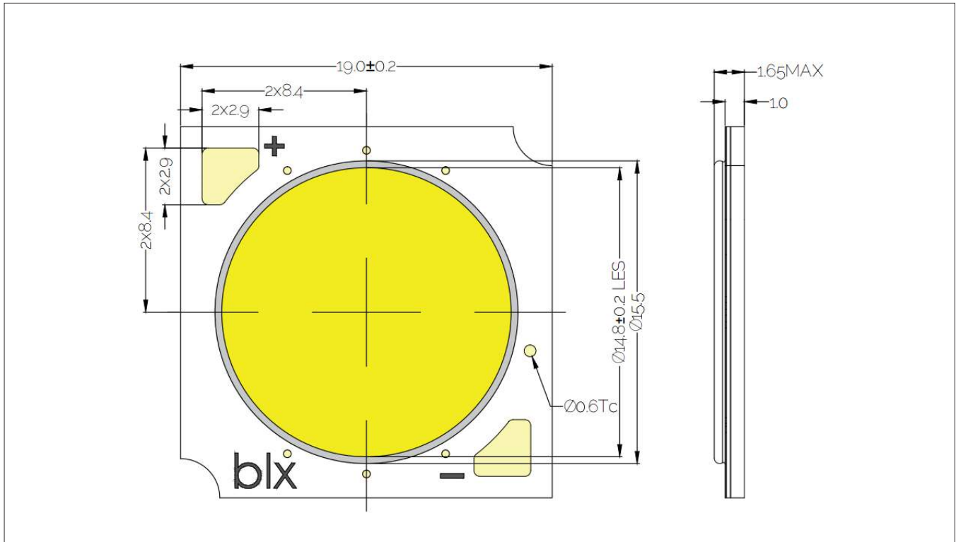
Figure 16: V13 LED Array
