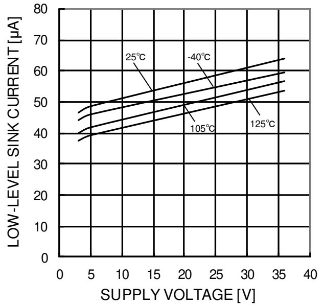
Figure 83. Low Level Sink Current - Supply Voltage (OUT=0.2V)
