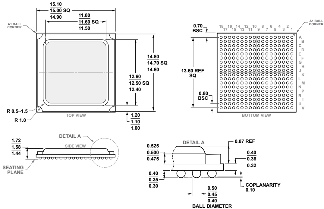
COMPLIANT TO JEDEC STANDARDS MO-275-KKAB-1 Figure 100. 324-Ball Ball Grid Array, Thermally Enhanced [BGA_ED] (BP-324-3) Dimensions shown in millimeters
