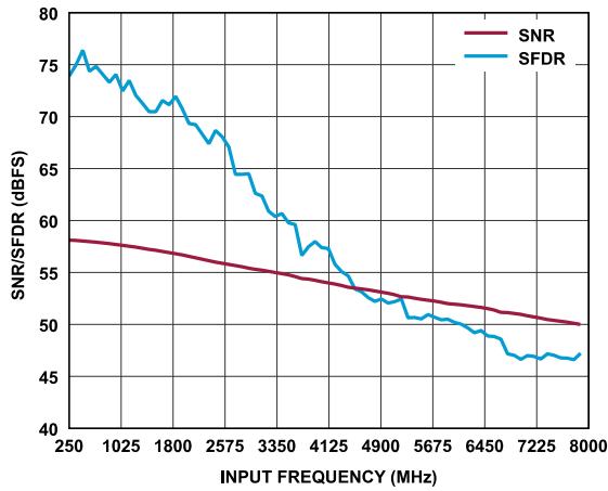
Figure 96. SNR and SFDR vs. Input Frequency with A_{IN} = -1 dBFS
