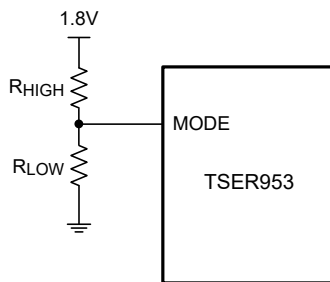
Figure 7-7. MODE Configuration
