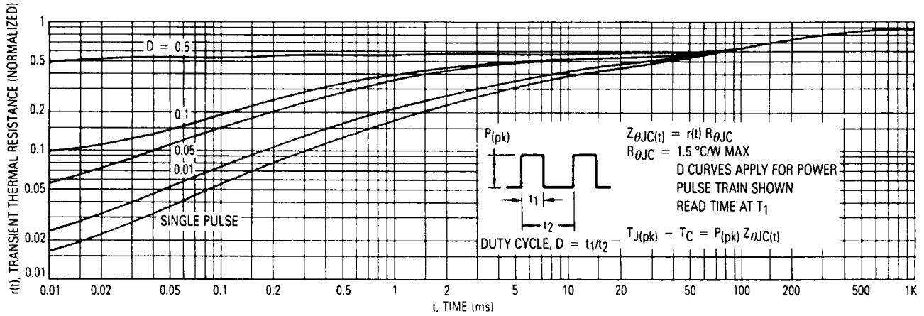
Figure 16. Thermal Response
