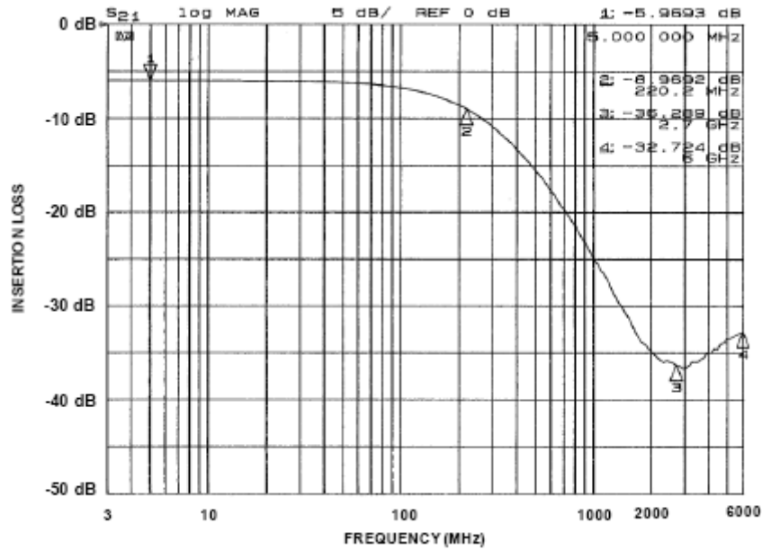
Figure 2. Insertion Loss vs. Frequency (A1-C1 to GND B1)
