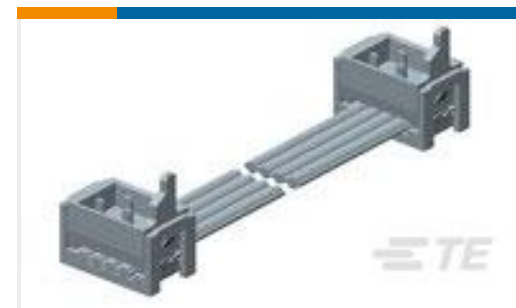
TE Part #2205061-2 CA MICRO-MATCH MOW-MOW 6POS
