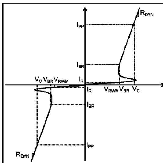
Fig. 8.1 Definitions of Electrical Characteristics
