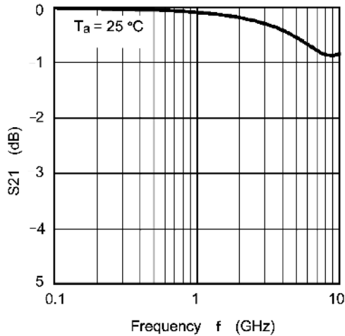
Fig. 9.5 S_{21} - f
