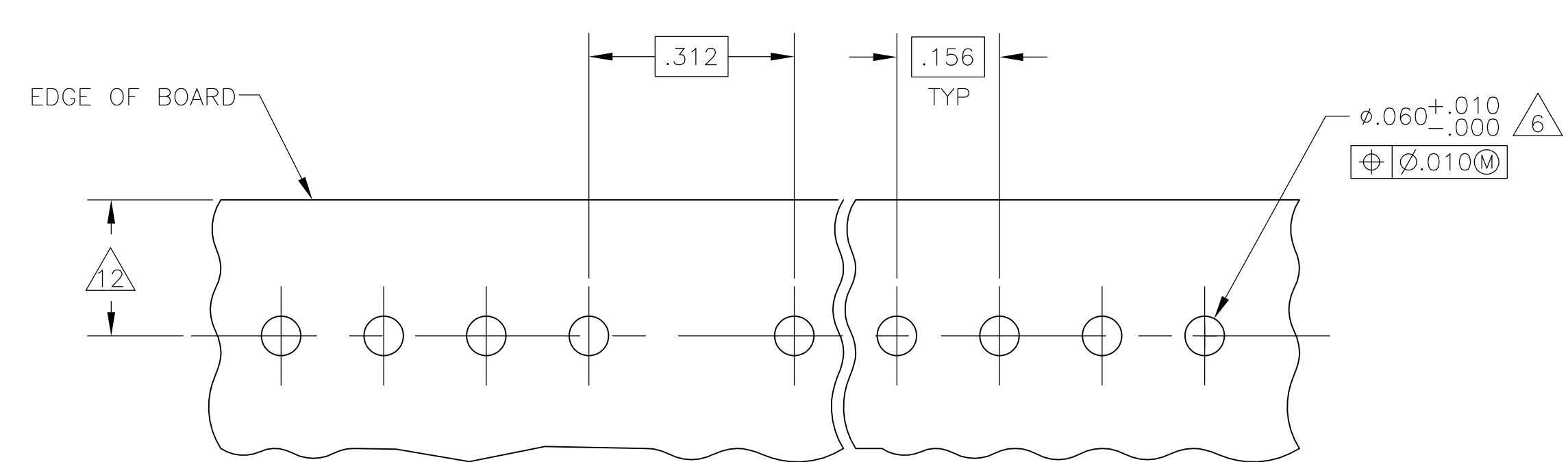
(C1) RECOMMENDED MOUNTING HOLE PATTERN (2) FOR .109 ± 0.016 THICK P.C. BOARD
