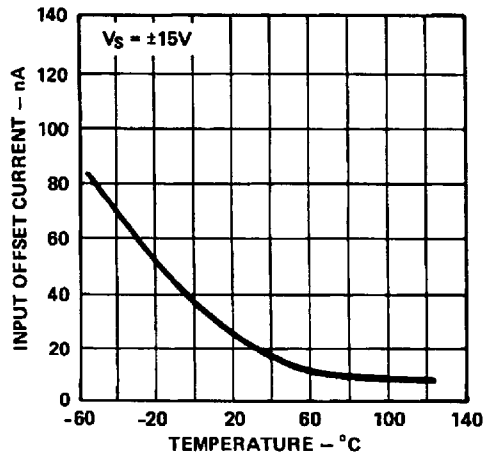
Figure 2. Input Offset Current vs. Temperature
