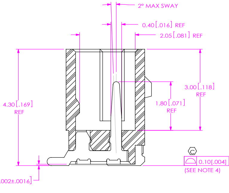
SECTION "A"-"A" SCALE 12 : 1
