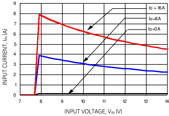
Figure 7. Input Voltage vs. Input Current ( V_o = 3.3\text{Vdc} ).
