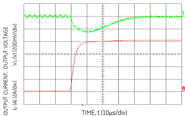
Figure 12. Transient Response to Dynamic Load Change from 50% to 100% of full load ( V_o = 3.3\text{Vdc} , C_{ext} = 2 \times 150\ \mu\text{F} Polymer Capacitors).
