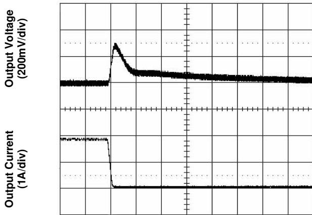
Time – t (100μs/div)
