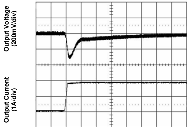
Time – t (100μs/div)
