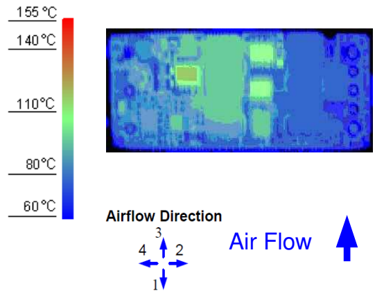
Figure 12. Thermal Image for Airflow Direction 3 (6.4A output, 85°C ambient, 200 LFM, typical V_{in} , open frame, socket interface)
