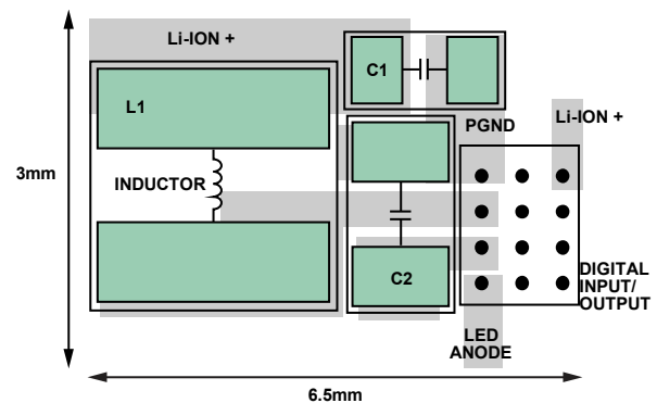
Figure 2. PCB Layout
