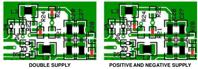
Figure 16. Double Supply Configuration with 0 Ω Resistors (Red)
